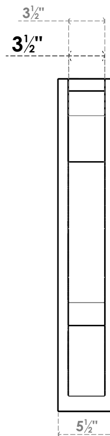
FRONT PROFILE
